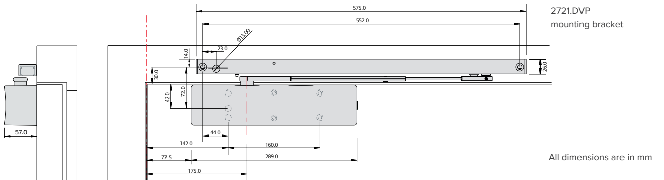
Electromagnetic hold-open variant (all other dimensions as standard closer)
